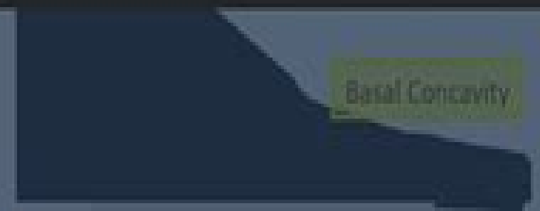
Fig. Ideal Hillslope Profile
