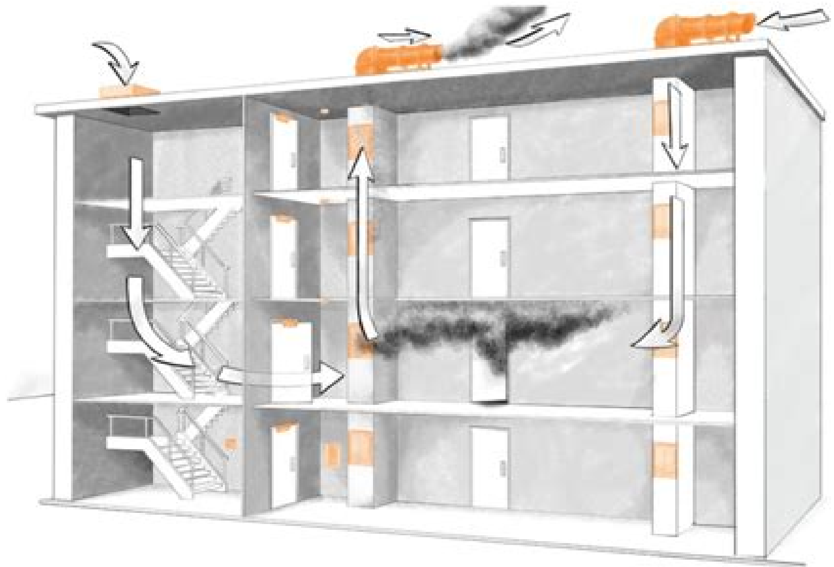
Figure 1: A sketch illustrating the application of a smoke-control system to extend the time available to evacuate a building safely in the event of a fire. This uses mechanical smoke shafts that provide substantial space-saving benefits compared with natural systems, and can be implemented in buildings with longer escape-route corridors
