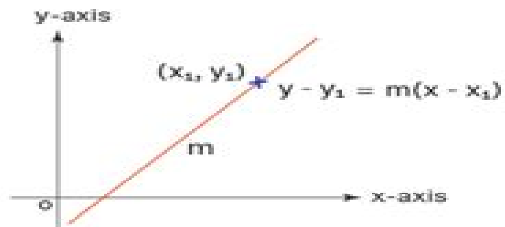
Point Slope Form
