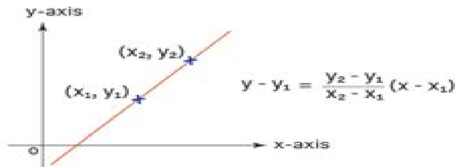
Two Point Form
