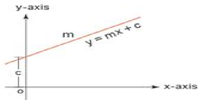
Slope Intercept Form
