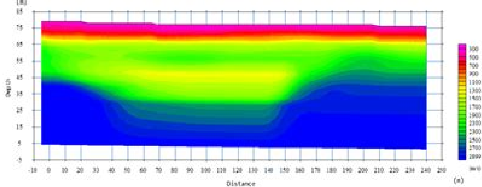
(a) Seismic refraction tomography model
