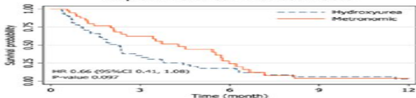
Kaplan-Meier survival estimates
