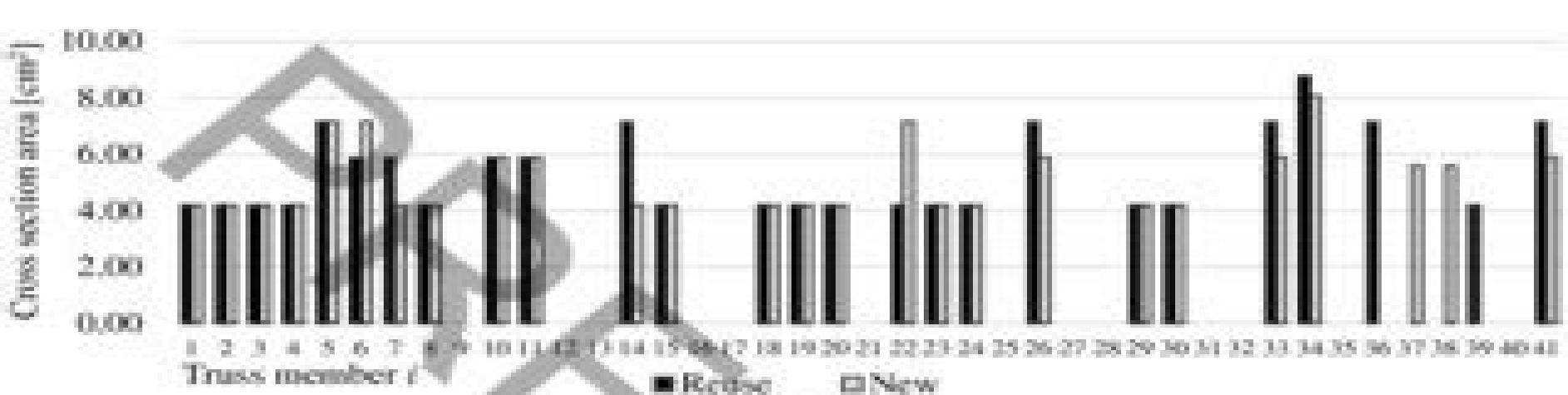
Fig. 16. Bridge truss – cross-section areas – reuse ( min E ) and new material system
