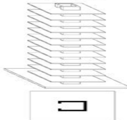
Outrigger Frame System
