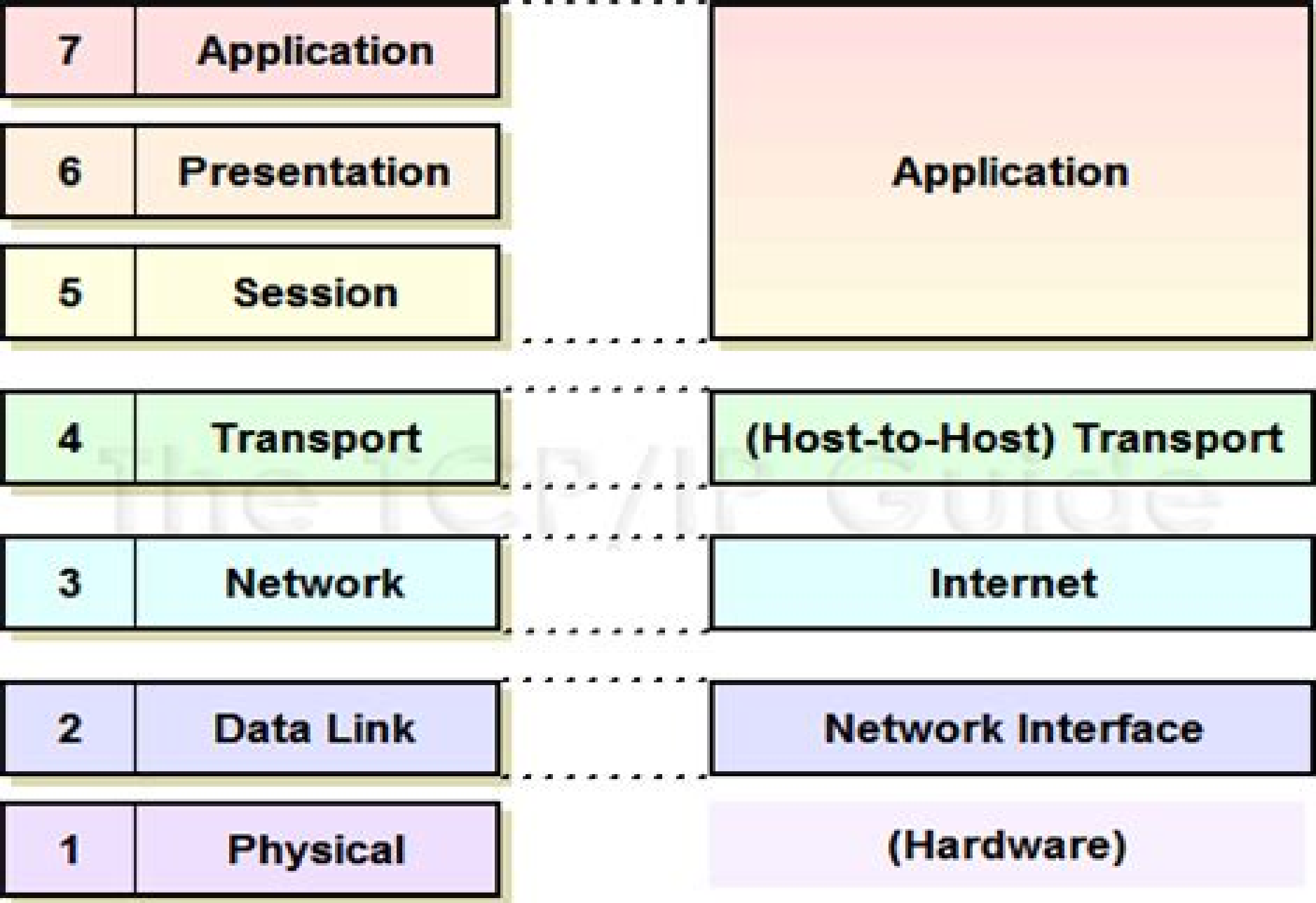
OSI Model
