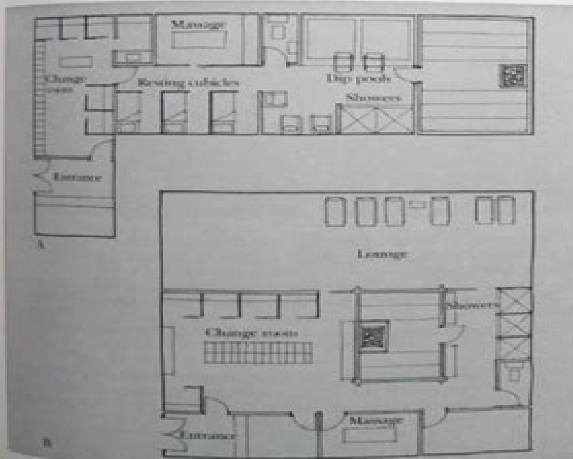
Fig. 2.16 Alternative layout for large mixed installations. A, through-draught layout, and B, circular system. Separate facilities are usually provided for males and females, sometimes with a common reception area. The alternative is to have one installation with facilities allocated to each sex.
