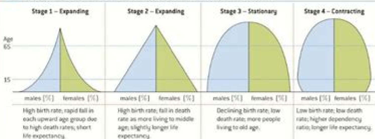
▲ Figure 8.1.15 The four shapes of population pyramids
