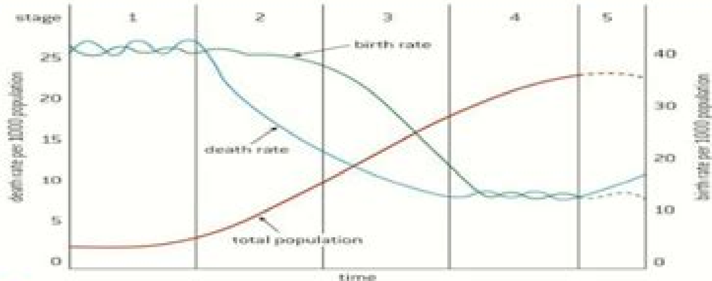
▲ Figure 8.1.14 The demographic transition model
