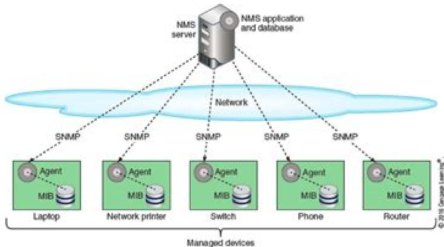
Figure 9-2 Network management architecture
