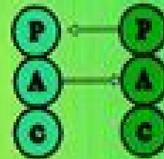
Parallel
