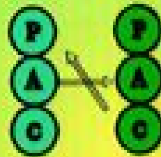
Crossed
