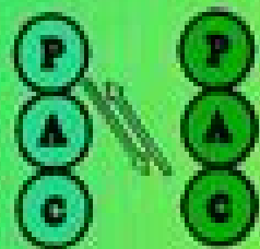
Complementary
