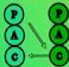
Angular
