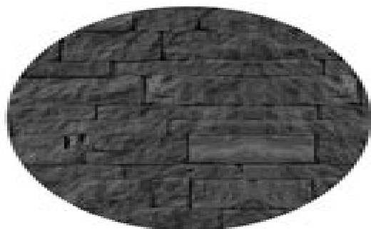
Basalt
