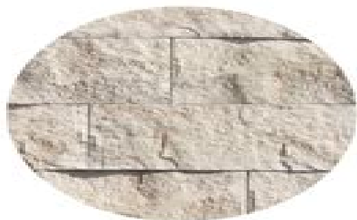
Limestone
