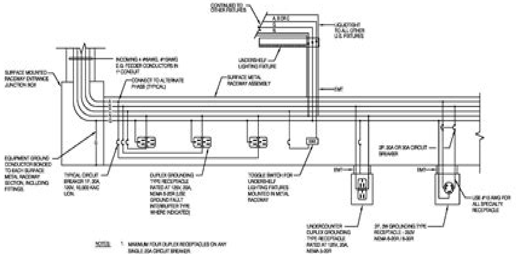
SURFACE METAL RACEWAY WIRING DETAIL NO SCALE
