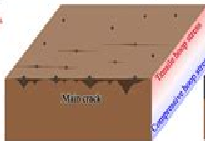
Stage 3: Coalescence of small cracks and propagation of SCC
