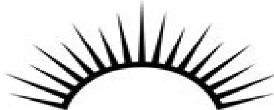
sunrays constancy
