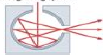
Integrating sphere
