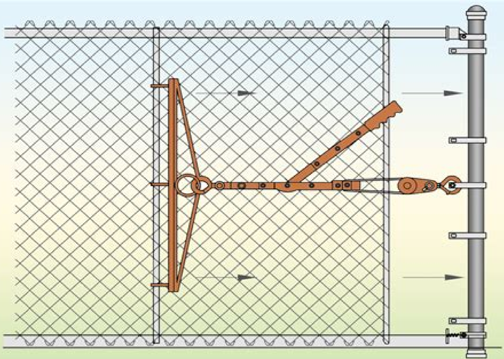
Stretching Fence Fabric
