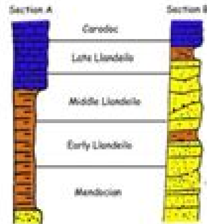
Geochronologic Correlation
