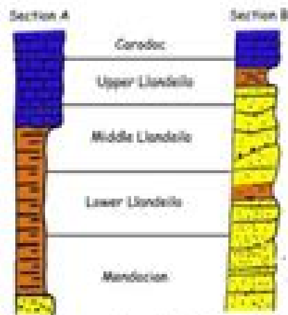
Chronostratigraphic Correlation
