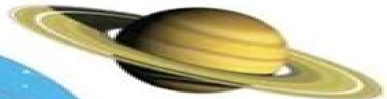
Saturn's rings
