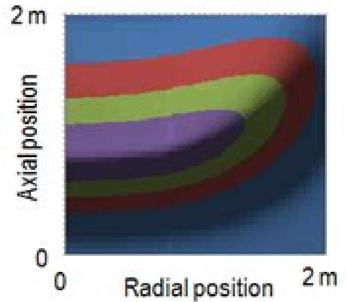
Flattened CANDLE
