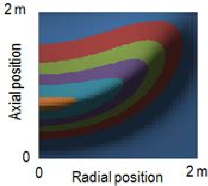
Original CANDLE
