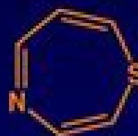
1,4-thiazepine
