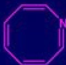
azocine
