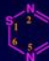
6H-1,2,5-thiadiazine
