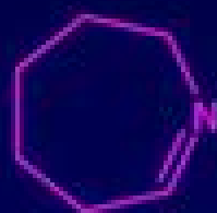
3,4,5,6-tetrahydro-2H-azepine
