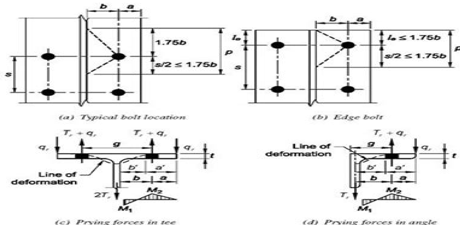
Fig. 9-4. Illustration of variables in prying action calculations.
