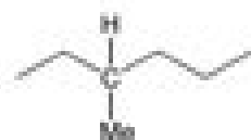
3-methylhexane
