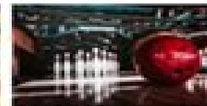
Bowling
