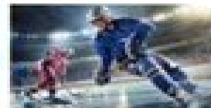
Ice Hockey
