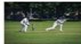
Cricket
