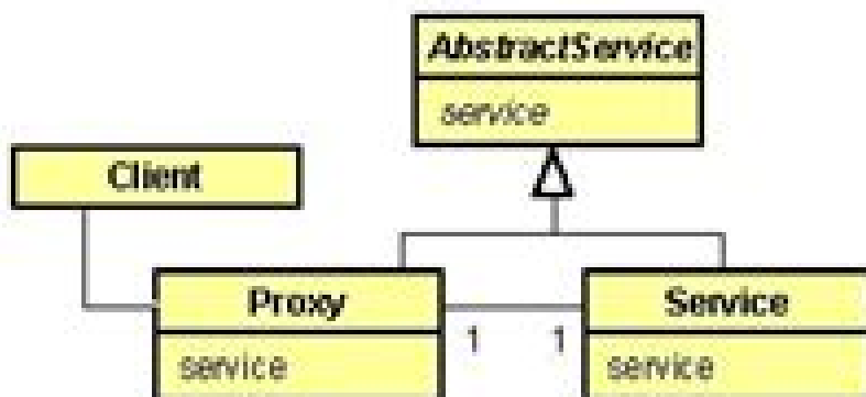
The Proxy Pattern
