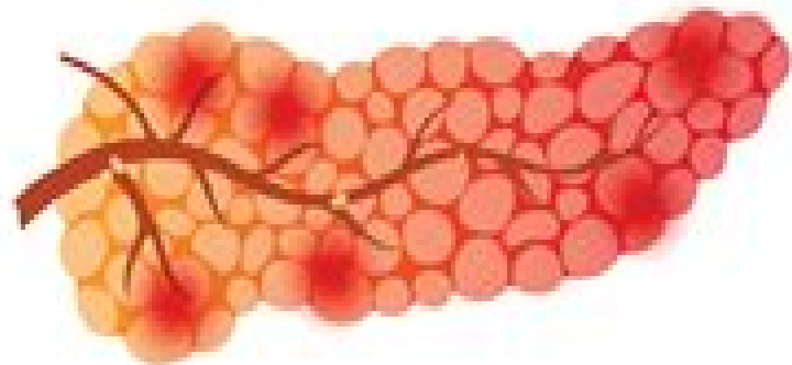
Chronic pancreatitis
