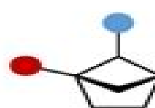
bioisostere
