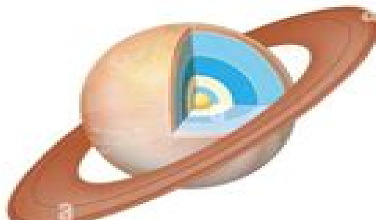
Saturn
