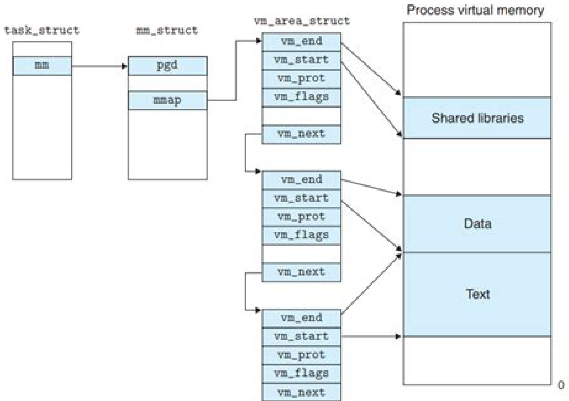
Figure 9.27 How Linux organizes virtual memory.
