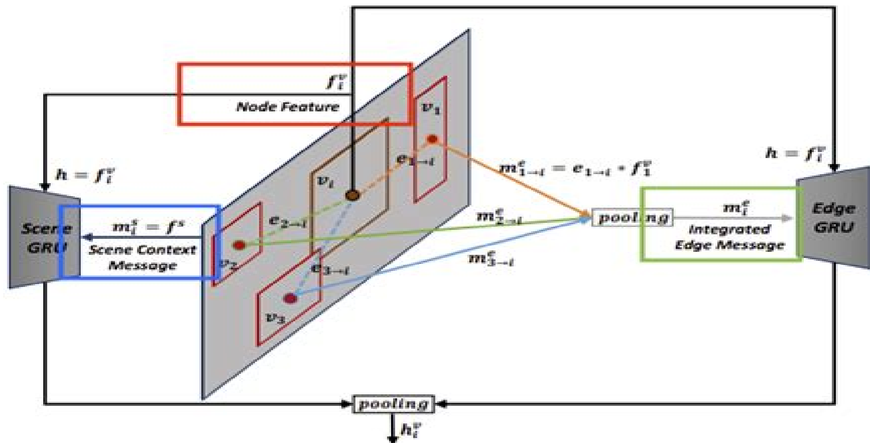
Figure 5. Structure Inference. For object v_i , the input of scene GRU is scene context message m_i^s , and the initial hidden state is the node v_i feature f_i^v . For message m_{1 \rightarrow i}^e from node v_1 to node v_i is controlled by edge e_{1 \rightarrow i} . These messages from all other objects are integrated as m_i^e to input the edge GRU. The initial hidden state of edge GRU is also f_i^v . Then these two sets of GRU output ensemble together as eventual updated node state.
