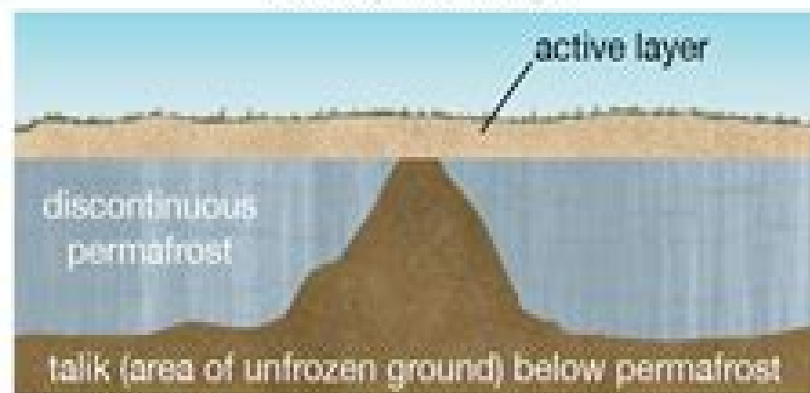
open-system pingo
