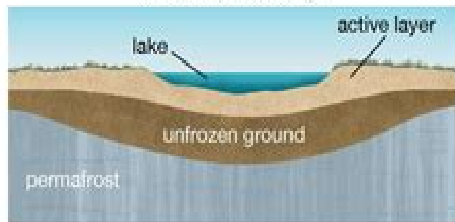
closed-system pingo
