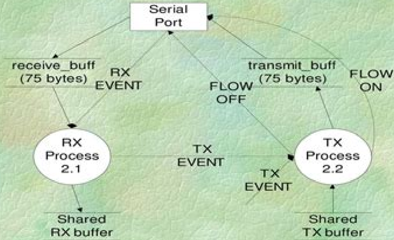
Serial Task Data Flow Diagram Level 1
