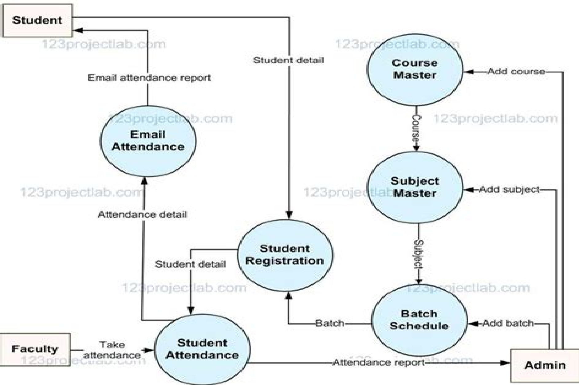
Level-1 DFD for Student Attendance Management System
