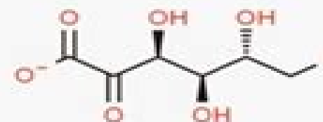
2-Ketogluconate
