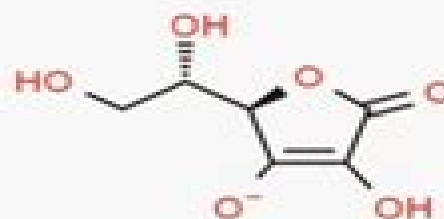
Ascorbate
