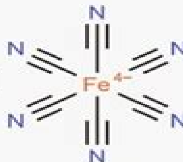
Ferrocyanide
