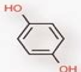
Hydroquinone
