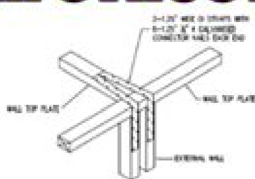
INTERNAL BRACING WALL TO EXTERNAL WALL CONNECTION
