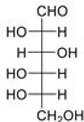
L-glucose
