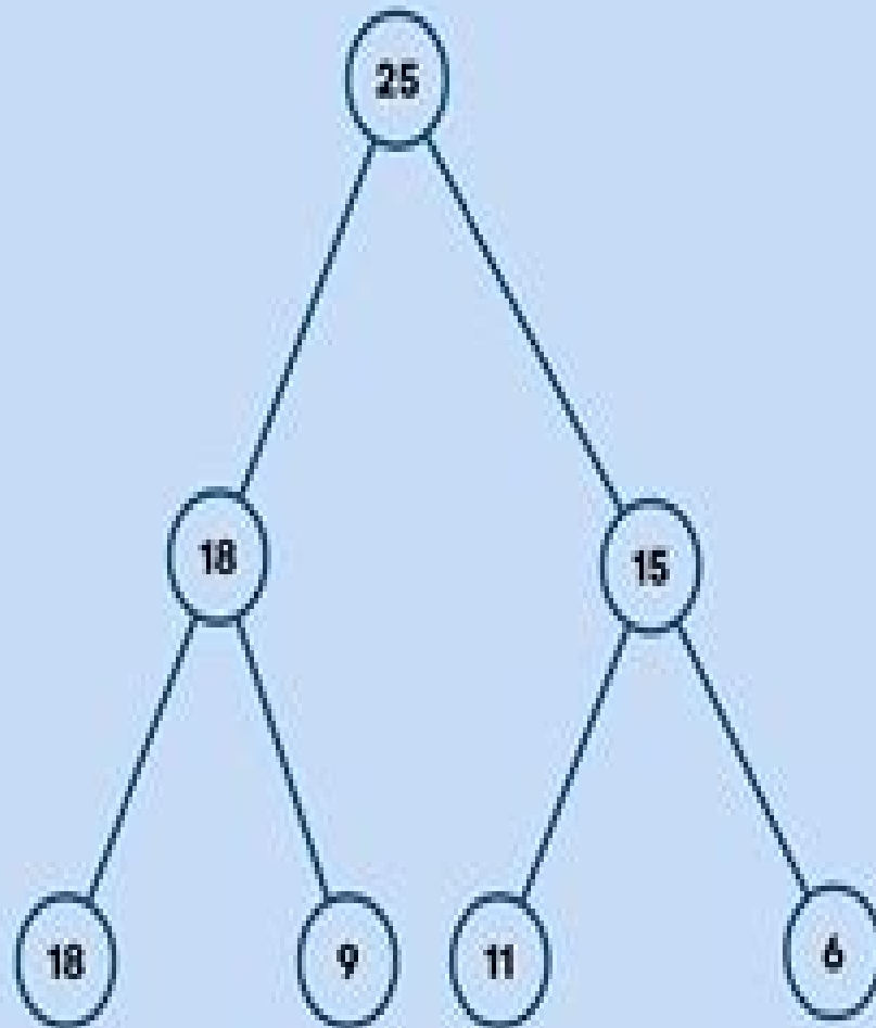
MAX HEAP
