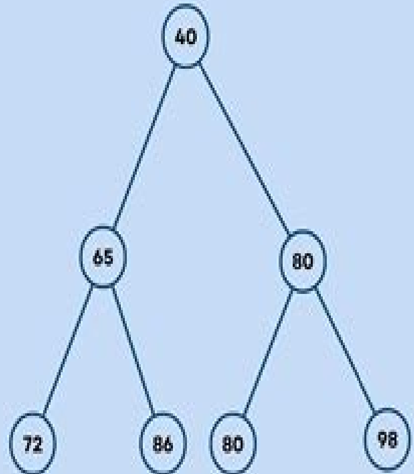
MIN HEAP
