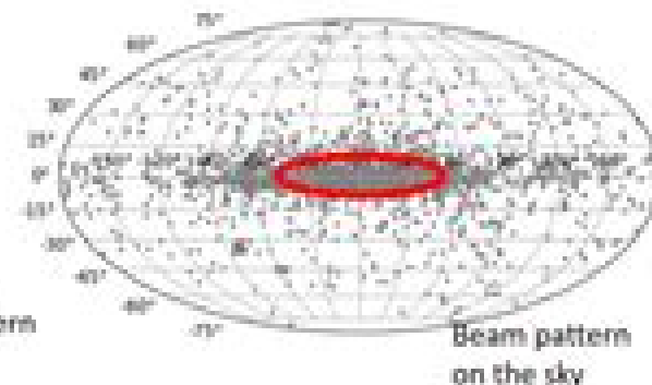
Sky Distribution of Known Pulsars
