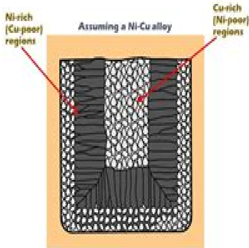
Figure: Characteristic grain structure in an alloy casting, showing segregation of alloying components in center of casting.
