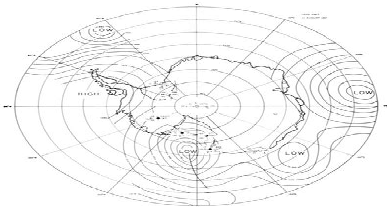
Fig. 14. 1200, August 11. Illustration of the blocking high situation.
