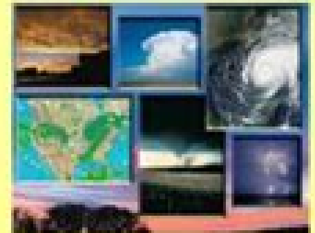
METEOROLOGY
