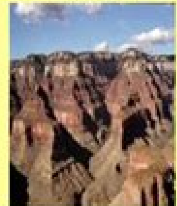
GEOLOGY
