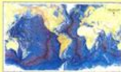
OCEANOGRAPHY
