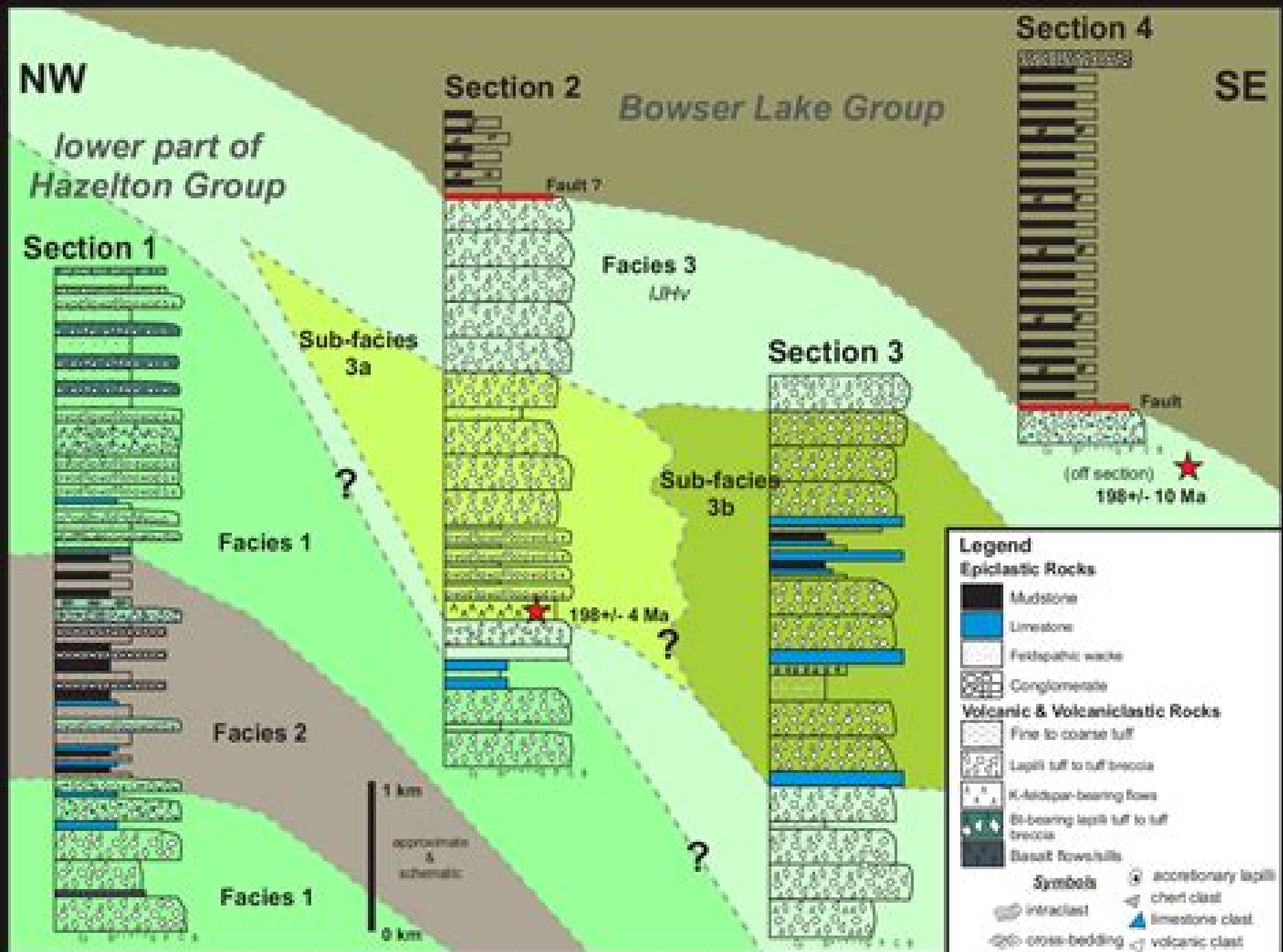
Fig. 1 Simplified generalized stratigraphic sections based on new data in the Vitreous River area outlines three volcanic-sedimentary facies and
