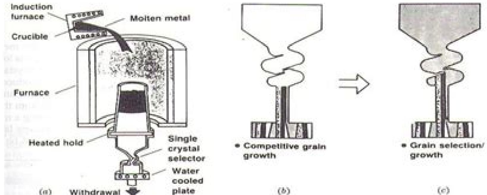
FIGURE 4.12 (a) A process schematic for producing a single-crystal gas turbine airfoil. (b) Starter section of casting for producing a single-crystal airfoil showing competitive growth during solidification below the single-crystal selector ("pigtail"). (c) Same as (b) but showing the survival of only one grain during solidification through the single-crystal selector. (After Pratt and Whitney Co.)
