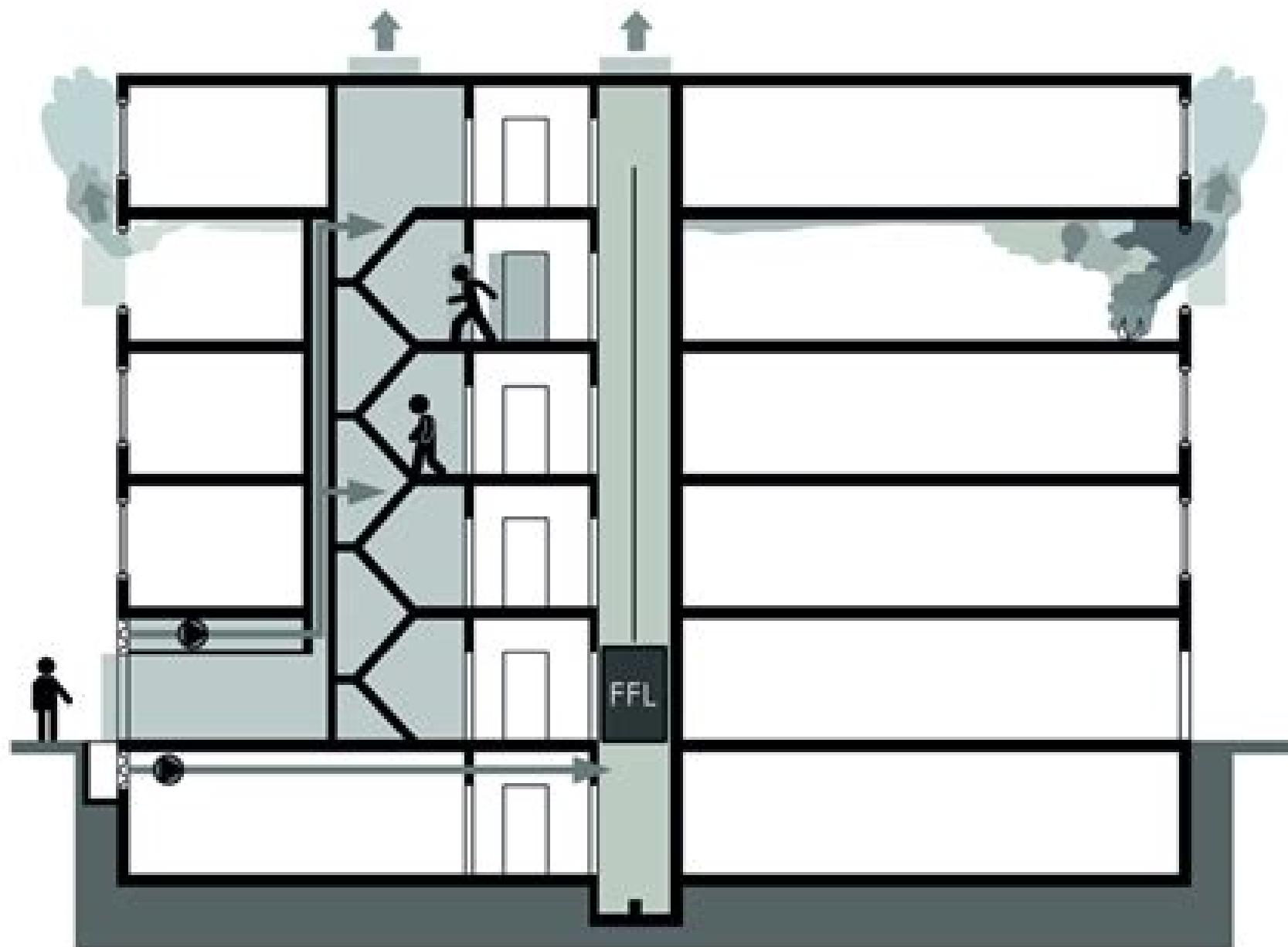
Figure 1: A typical pressurisation system with staircase and firefighters' lift-shaft protection, and air release in the façade(s) (Source: BS EN 12101-13 2022)
