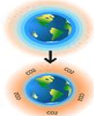
Greenhouse Effect
