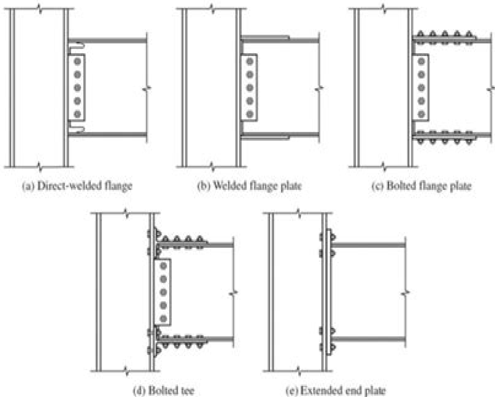
Figure 2 Moment Connections
