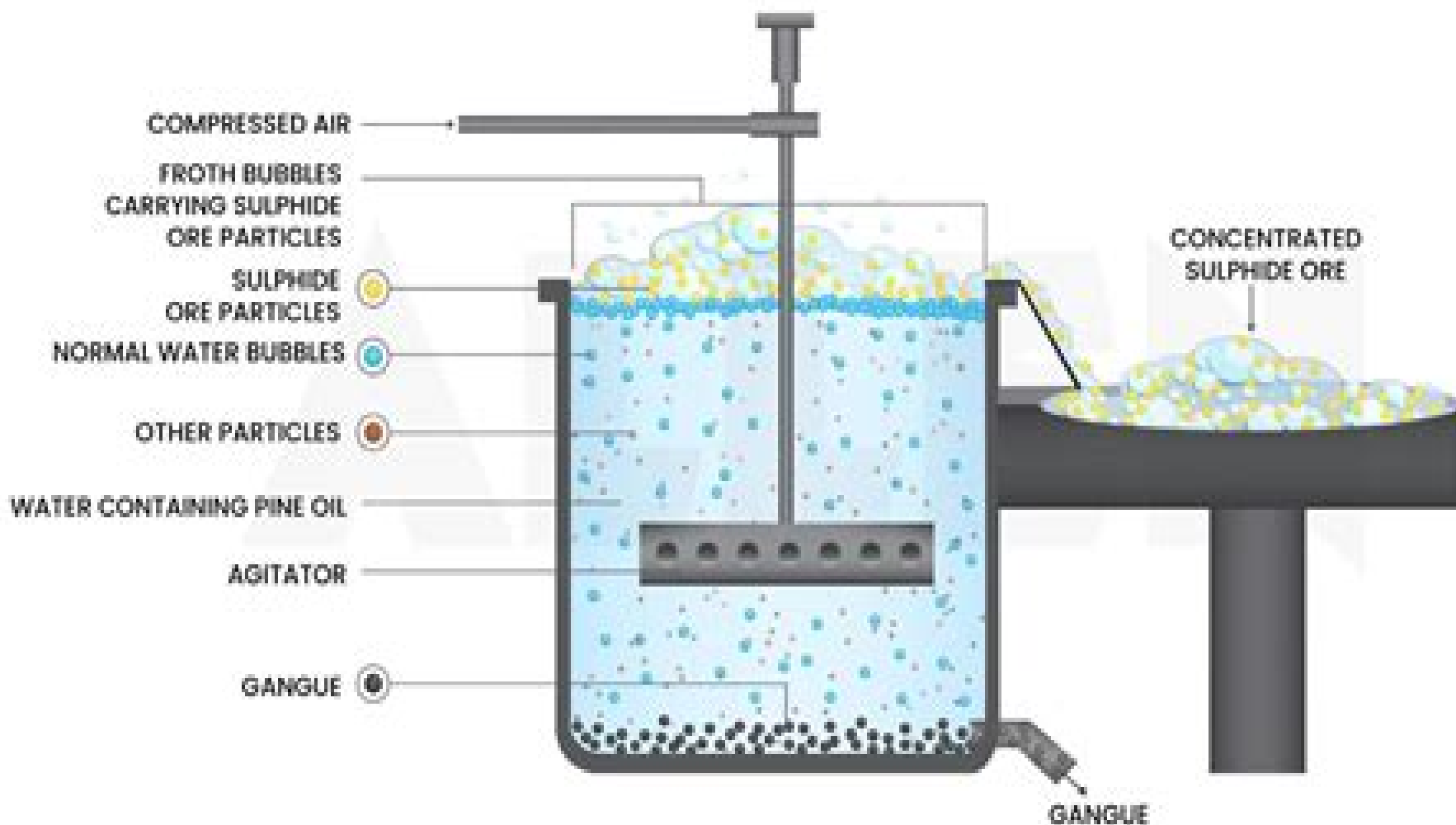
Froth flotation
