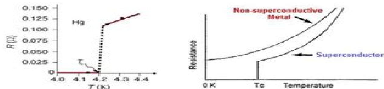
(a) Plot of the resistance of Mercury vs. temperature, showing sudden decrease of the critical temperature, at 4.2 K. (b) Combined resistance vs temperature graphs of a non superconducting material and a superconducting material.
