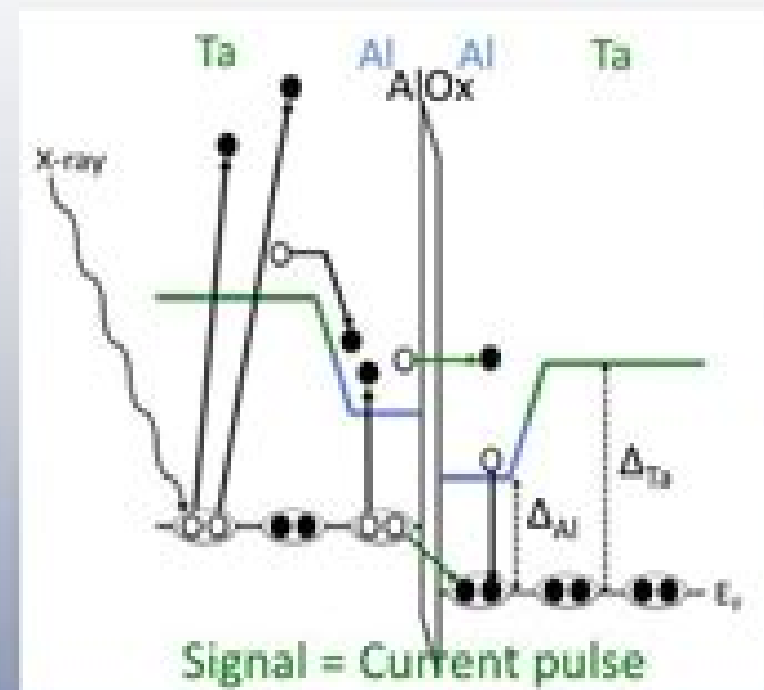
STJ Operating Principle
